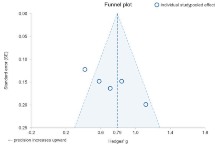
Figure 6. Funnel Plot
